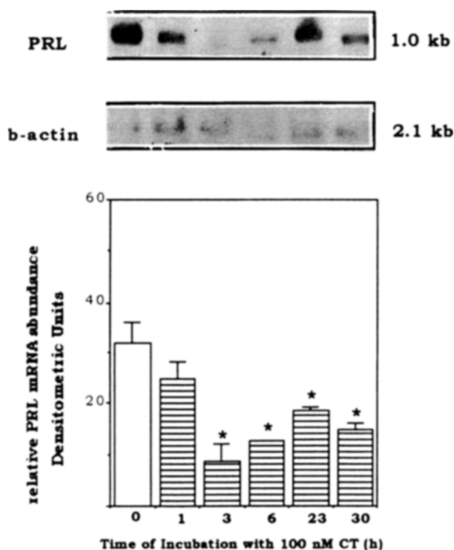
Figure 3 Time course of sCT action on PRL mRNA levels in GH 3 cells. GH 3 cells were incubated with 100 nM sCT for various time periods. Total cellular RNA (20 µg) was subjected to Northern blot analysis and probed sequentially with 32 P-labelled PRL and β-actin cDNAs. A representative autoradiogram depicting PRL mRNA signals after 2-day exposure (upper panel), and β-actin mRNA signal after 1-day exposure (lower panel). The autoradiograms were scanned by laser densitometry and absorbances for the bands were calculated. Relative PRL mRNA levels are presented as ratio of PRL mRNA to β-actin mRNA × 100. The data were analysed by one way ANOVA and the significance was derived by Newman-keuls test. * P < 0.05
