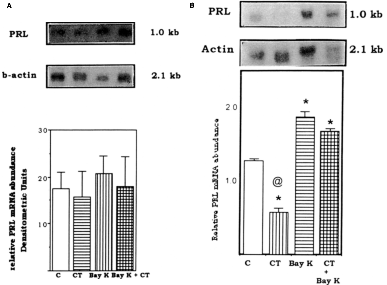
Figure 8 Effect of CT on \text{Ca}^{2+} -induced PRL mRNA levels in \text{Ca}^{2+} -deprived GH 3 cells. (A) GH 3 cells were preincubated in SFM ( \text{Ca}^{2+} -free, serum-free chemically-defined medium) for 2 days and then treated with agonists as described in the Methods section. Total cellular RNA (20 \mu\text{g} ) was subjected to Northern blot analysis and probed sequentially with ^{32}\text{P} -labelled PRL and \beta -actin cDNA probes. A typical autoradiogram presents the PRL mRNA signals in top panel (4-day exposure); and \beta -actin mRNA signal in lower panel (2-day exposure). Autoradiograms from four independent experiments were scanned by laser densitometry. Relative PRL mRNA levels are presented as arbitrary densitometric units. The data were analysed by t -test. * P < 0.01 (significantly different from control). (B) GH 3 cells were preincubated in SFM ( \text{Ca}^{2+} -free, serum-free chemically-defined medium) for 2 days and then incubated with 0.5 mM \text{CaCl}_2 and other agonists for 6 h. Total cellular RNA (20 \mu\text{g} ) was subjected to Northern blot analysis and probed with ^{32}\text{P} -labelled PRL cDNA. Top panel presents a typical autoradiogram depicting PRL mRNA signal (3-day exposure). \beta -actin cDNA in the same blot is presented in the lower panel (2-day exposure). Autoradiograms from four independent experiments were scanned by laser densitometry. Mean relative PRL mRNA levels \pm SEM are presented as arbitrary densitometric units. The data were analysed by t -test. * P < 0.01 (significantly different from control); @ P < 0.03 (significantly different from Bay K).
