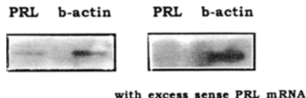
Figure 4 Characterization of nuclear run-on assay: displacement of nuclear PRL mRNA with sense PRL mRNA. Primary transcripts from GH 3 cell nuclei were labeled with [ 32 P]UTP in a nuclear run-on assay. The labeled nuclear RNAs were then extracted and hybridized in the presence and absence of excess sense PRL mRNA (1 µg). Left panel shows PRL mRNA hybridization signal obtained in the absence of exogenously added sense PRL mRNA. Right panel shows the PRL mRNA signal in the presence of 1 µg sense PRL mRNA. The presence of sense PRL mRNA during hybridization caused an almost complete extinction of PRL mRNA signal. β-actin mRNA signal was unaffected by the presence of sense PRL mRNA
