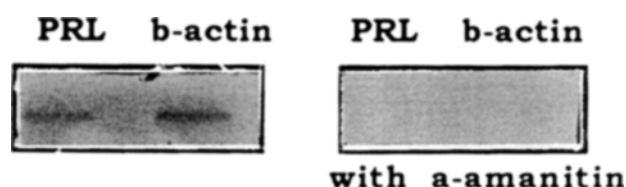
Figure 5 Characterization of nuclear run-on assay: effect of α-amanitin on PRL gene expression. To estimate the extent of RNA polymerase II-independent gene transcription, GH 3 cell nuclei were incubated with/without α-amanitin (2 µg/ml) during elongation of primary transcripts. Nuclear RNAs were then extracted and hybridized with Nytran strips containing PRL and β-actin cDNA inserts. A typical autoradiogram presents the hybridization signals under both conditions. α-amanitin caused a dramatic decline in incorporated radioactivity (by 80–85%). A similar decline was also observed in PRL and β-actin transcripts
